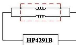
Common mode
